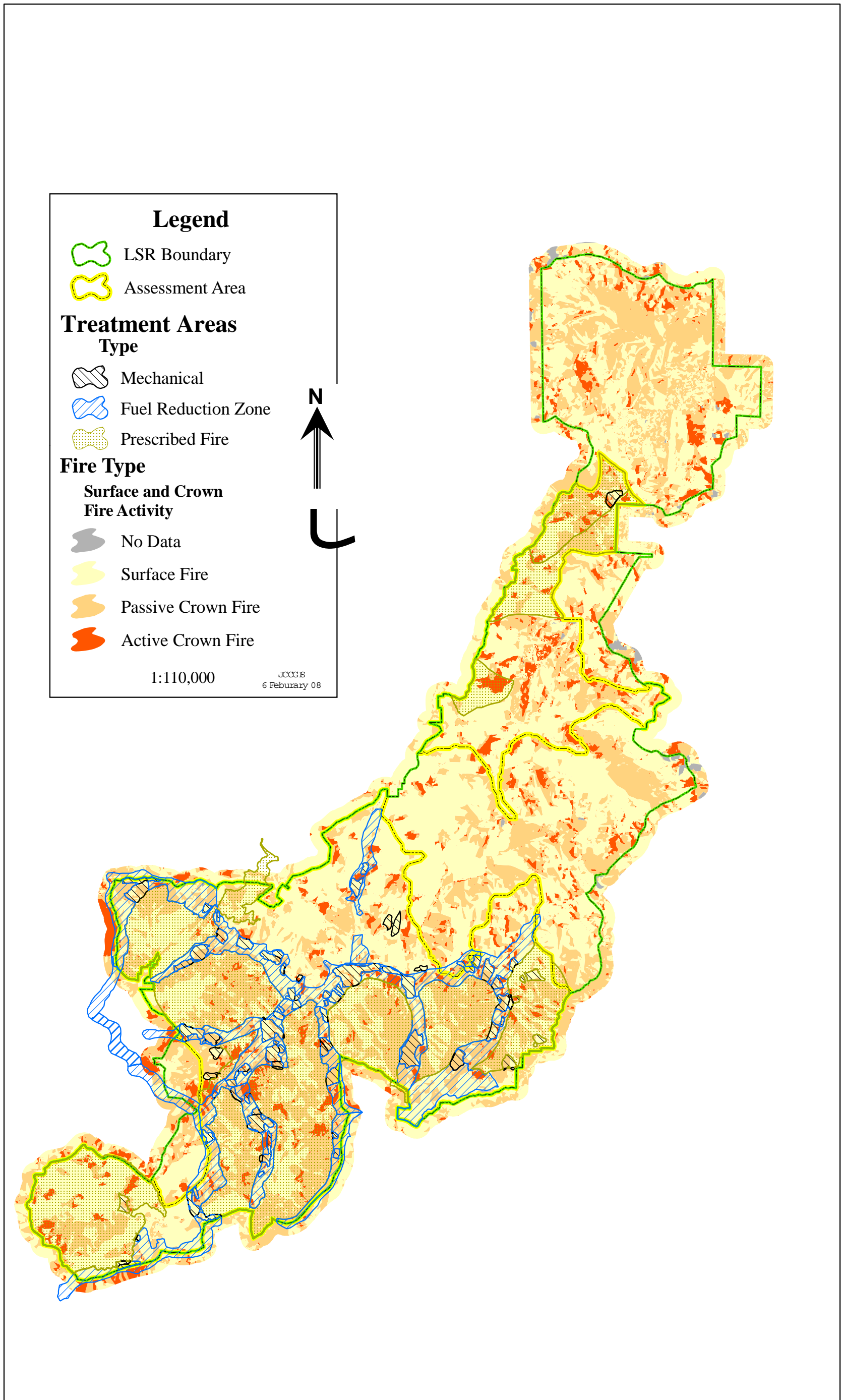
MAP A-3. FlamMap results showing surface and crown fire activity overlaid by proposed treatment areas.
